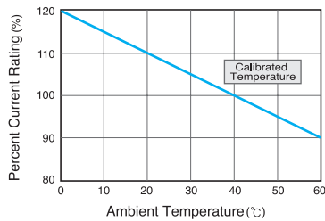
Ambient compensating curves
