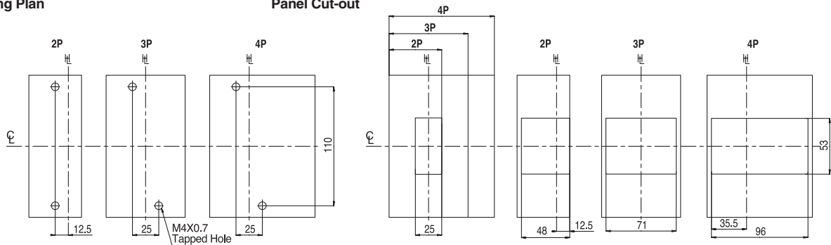
Drilling Plan
