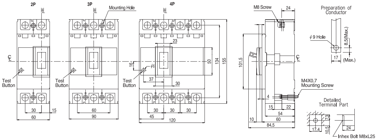
Drilling Plan
