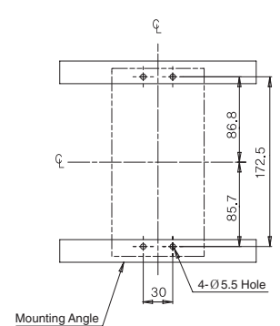
Drilling Plan
