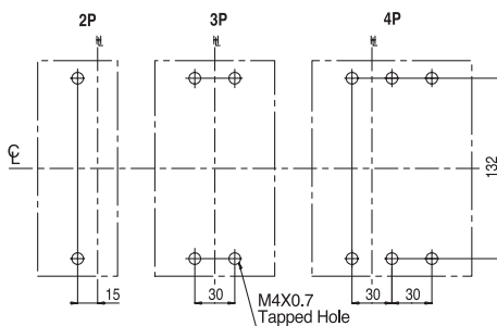
Drilling Plan
