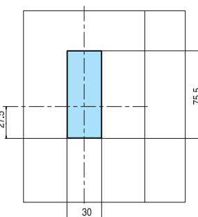
Panel Cut-out
