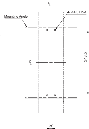
Drilling Plan
