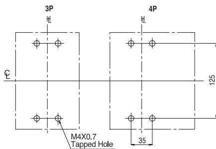
Drilling Plan
